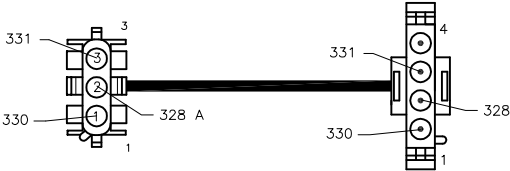
CONNECTOR AMP 1-480701-0 (CAP) TERMINAL AMP 350552-3 TERM FULL WALL CONTROLLER INPUT (TEACH PENDANT) INTERFACE DETAIL A (PIGTAIL PROVIDED WITH MODULE)
