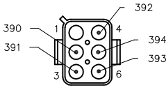
C-3 AMP 1-480704-0 (PLUG) AMP 350551-3 TERM
