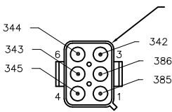
C-2 AMP 1-480704-0 (PLUG) PIN TERMINALS AMP 350552-3
