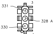
CONNECTOR AMP 1-480701-0 (CAP) TERMINAL AMP 350552-3 TERM FULL WALL CONTROLLER INPUT (TEACH PENDANT) INTERFACE DETAIL B
