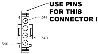
AUTOLOCK INTERFACE CONNECTOR AMP 1-480702-0 (PLUG) TERMINAL AMP 350552-3 TERM (QUEER CONNECTOR)
