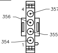
SENSOR CONNECTOR CONNECTOR AMP 1-480702-0 (PLUG) TERMINAL AMP 350551-3 TERM
