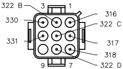
C-1 AMP 1-480706-0 CONN (PLUG) AMP 350551-3 TERM
