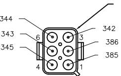
KEY SWITCH AMP 1-480704-0 (PLUG) PIN TERMINALS AMP 350552-3
